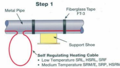
HEATING CABLES
